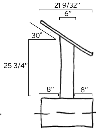
Side Elevation
